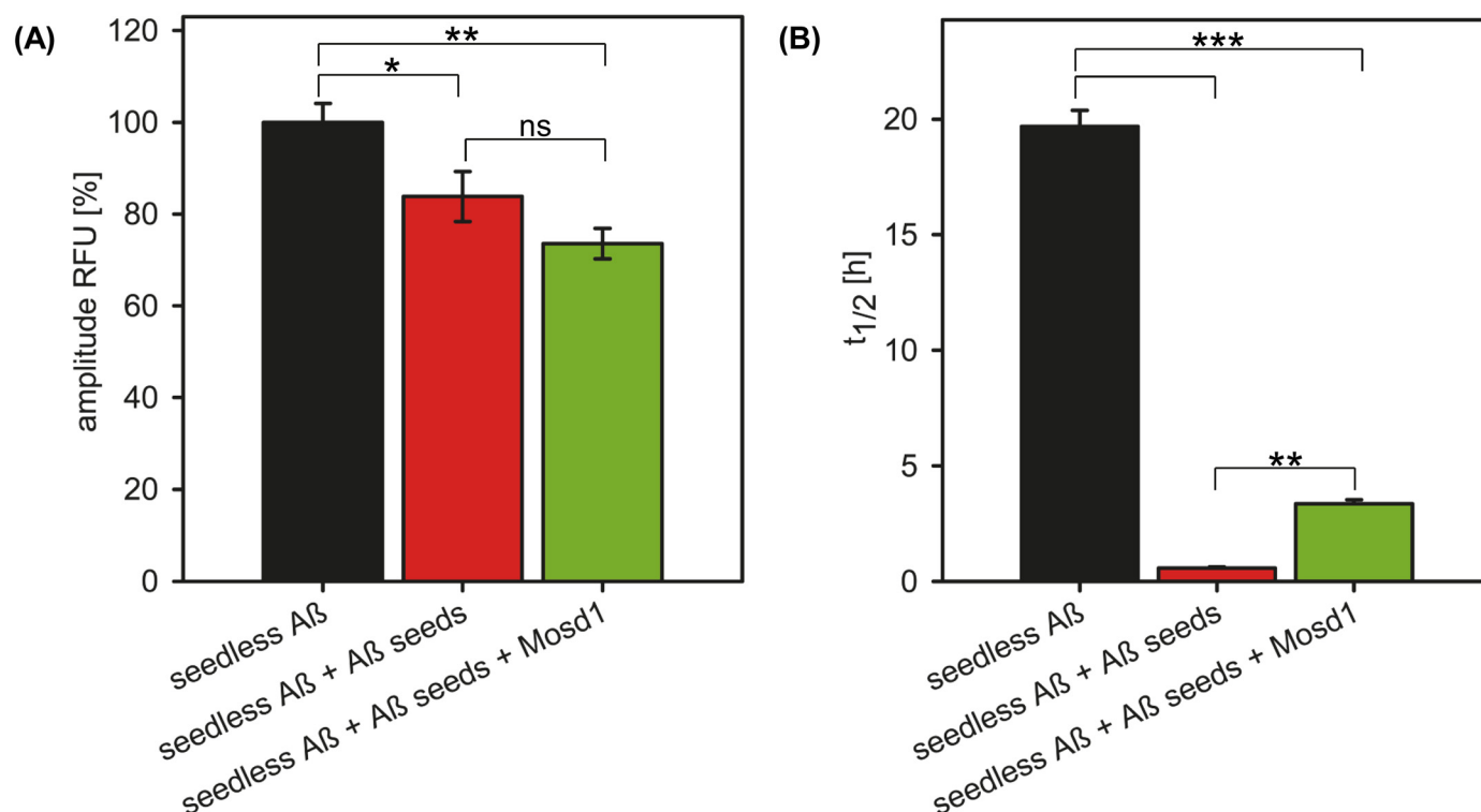
Fig 7. Reduction of seeded A \beta_{1-42} growth and fibrillar A \beta_{1-42} content. Seedless A \beta_{1-42} was incubated alone (black) or together with fibrillary A \beta_{1-42} seeds previously incubated with (green) or without (red) a fivefold molar excess of Mosd1. ThT (20 \mu M) was added to each sample in order to measure fibrillar content. The data were fitted with an asymmetric five parameter fit. The (A) amplitude of relative fluorescence (RFU) of fibrillated seedless A \beta_{1-42} served as 100% to which the other values were normalized. The (B) half-life ( t_{1/2} ), displaying the point in time, when half of the maximum ThT signal (i.e. fibrillar content) was reached. Statistical significance was determined by one-way ANOVA. Error bars display SEM. ns: p > 0.05 ; *: p \leq 0.05 ; **: p \leq 0.01 ; ***: p \leq 0.001 .
